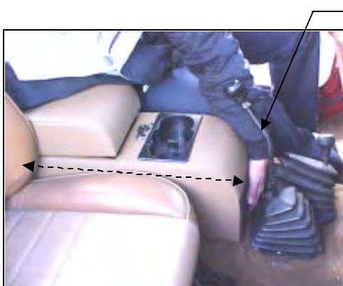
Figure 3 (13101.xx console shown for reference only. Installation is the same for 13102.XX)
