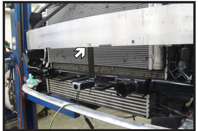
16. Optional: Attach the breakaway bracket to the bumper in the desired location with the supplied 1/4" hardware.
