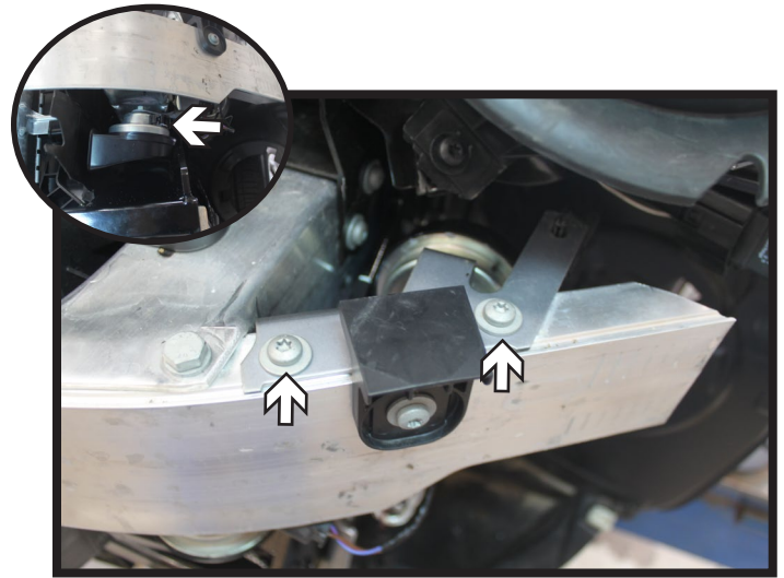
14. Leaving the lower horn loose, reinstall the bracket to the vehicle. After the bracket is reinstalled reattach the lower horn to the bracket.
