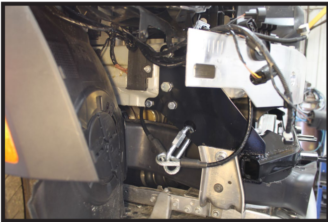
15. Attach the permanent baseplate safety cables to the convenience link hole on the baseplate. Secure the cables to a solid piece of the frame as described in the instructions included with the permanent baseplate safety cables. Be sure the safety cables do not rub against any hoses or moving parts. Do this on BOTH sides of the vehicle.
