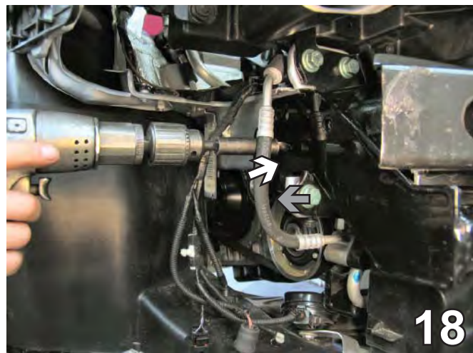
18. Using the baseplate as a template, drill the holes in the side of the frame rail with the 13/32" drill bit. Do this on both sides of the vehicle.
