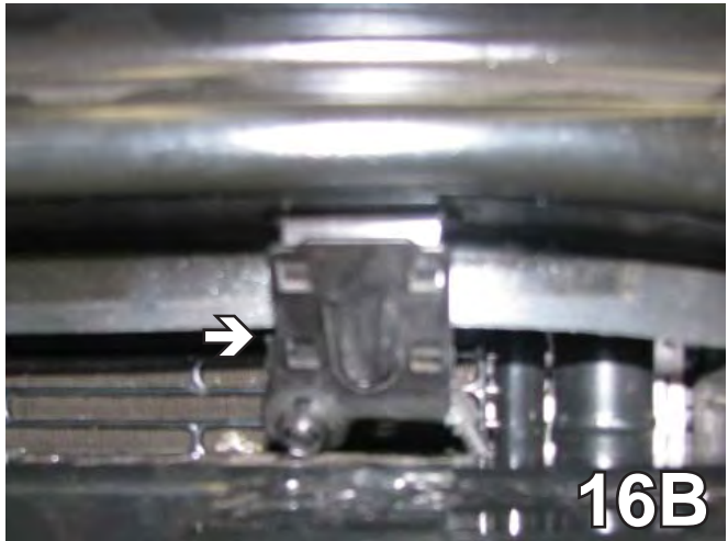
16. Cut the side piece off of the air temperature sensor (16A). Bend the metal piece back and snap the sensor into place (16B). This will prepare the area for the base plate installation.
