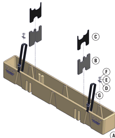
Ribs on buckle should face up. Thread strap through buckle as shown.
