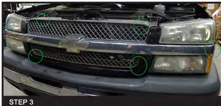
Loosen the grille mounting points
