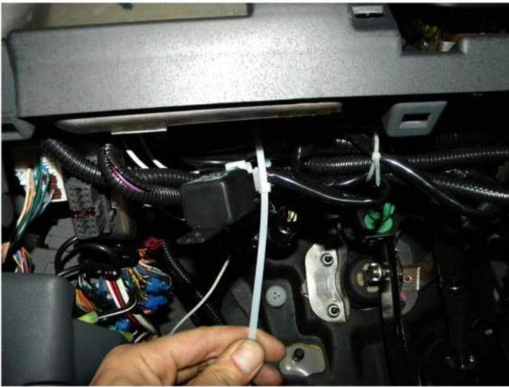
35. Zip the excess wire onto the factory wire harness
