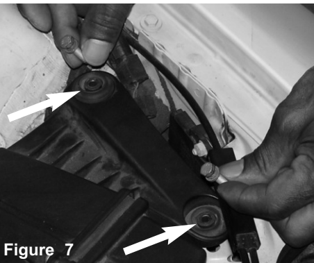
Figure 7 The 10mm bolts are now removed
