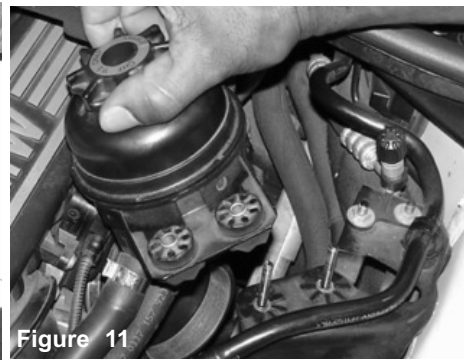
Figure 11 Without disconnecting the two lines, remove the reservoir bottle from the two studs.
