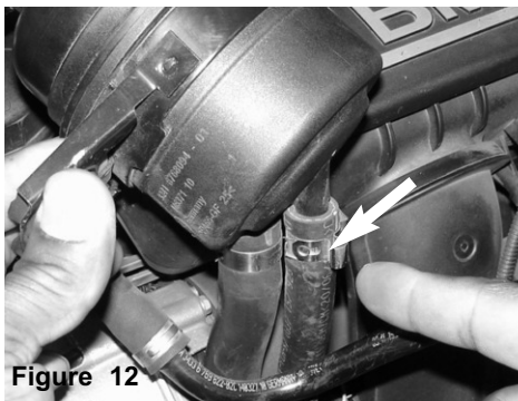
Figure 12 Note: This clamp will not be removed. The clamp will be rotated so that it will not interfere with the air intake.
