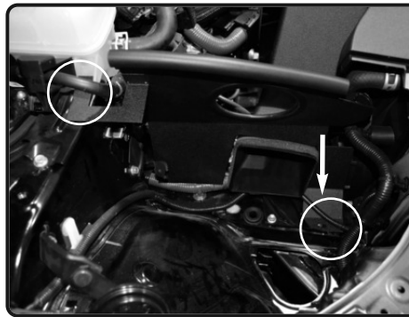
8" Rubber trim
