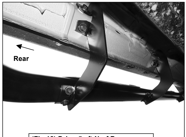
(Fig 12) Driver/Left Nerf Bar installed on Rear Mounting Bracket
