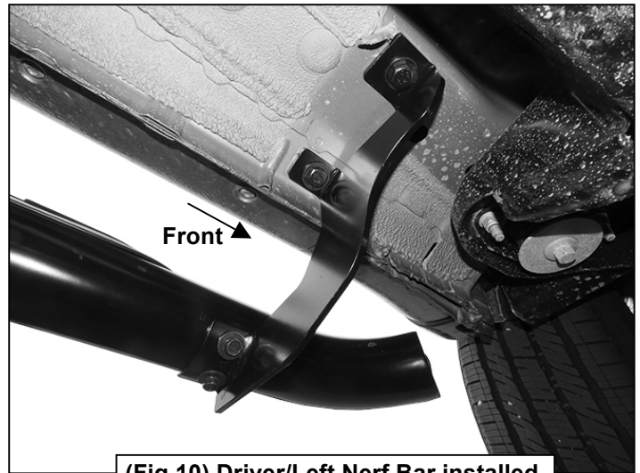
(Fig 10) Driver/Left Nerf Bar installed on Front Mounting Bracket
