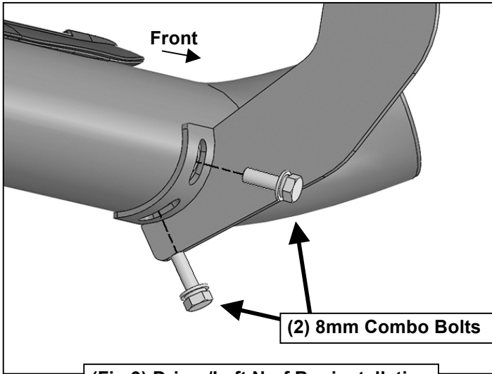
(Fig 9) Driver/Left Nerf Bar installation
