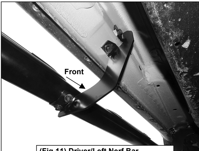
(Fig 11) Driver/Left Nerf Bar installed on Center Mounting
