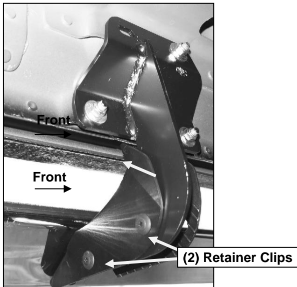
(Fig 5) Plastic Cover installation onto front bracket
