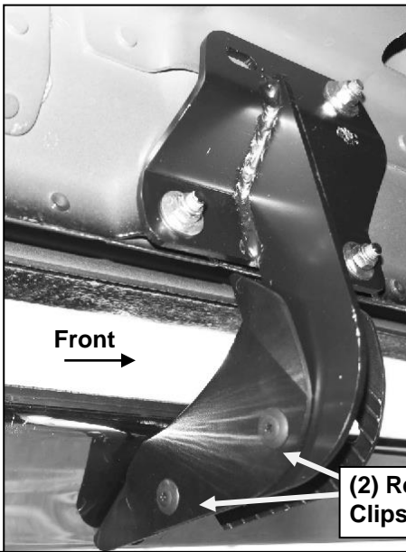
(Fig 5) Plastic Cover installation onto front bracket
