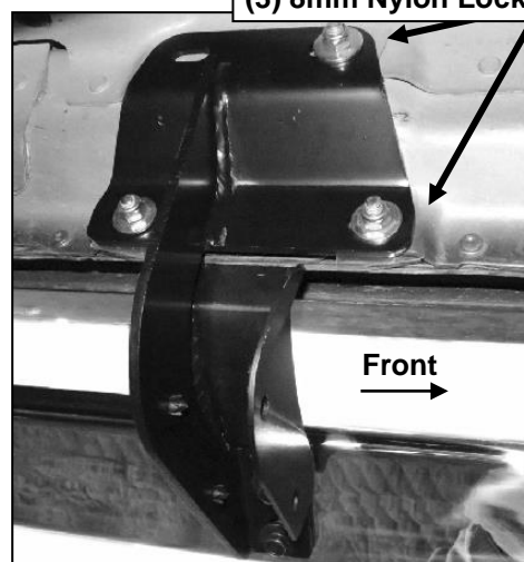
(Fig 4) Driver side front Bracket installation
