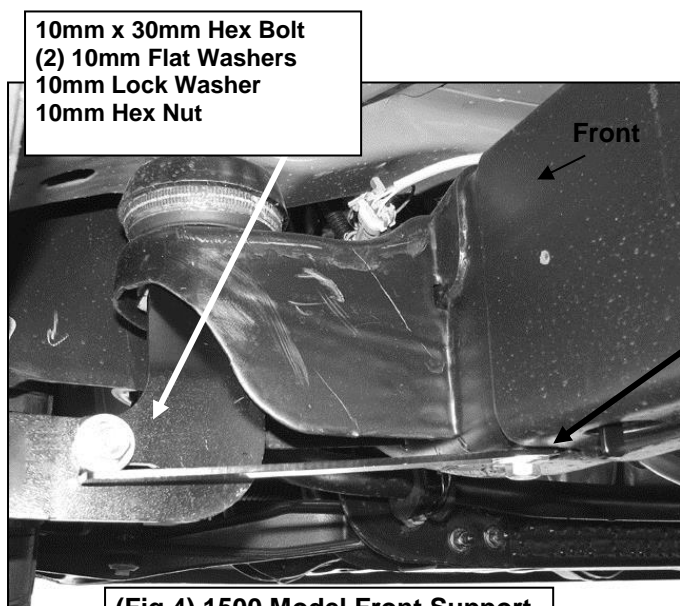
(Fig 4) 1500 Model Front Support Bracket Installation Pictured
