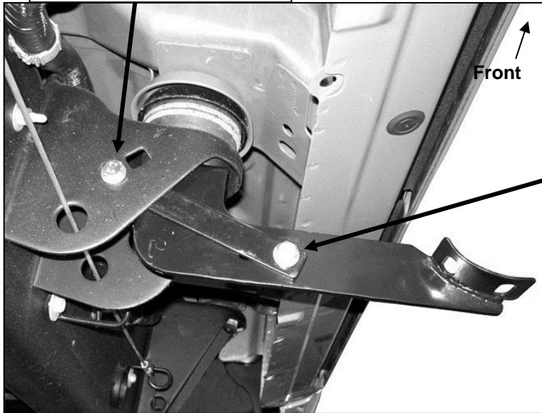
(Fig 6) 25-3500 Model Center Support Bracket Installation Pictured
