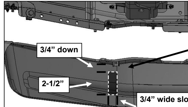
(Fig 13) Driver side-back of "tall" STD air dam illustrated. All measurements are for reference and example only, check all measurements before cutting air dam.
