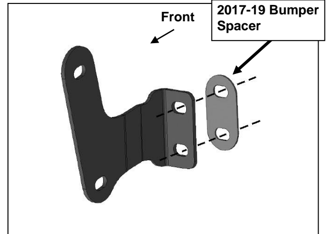
(Fig 4) On 2017-19 models only, attach driver/left Frame Bracket to Spacer and bumper. Do not install Bracket without Spacer on 2017-19 model years
