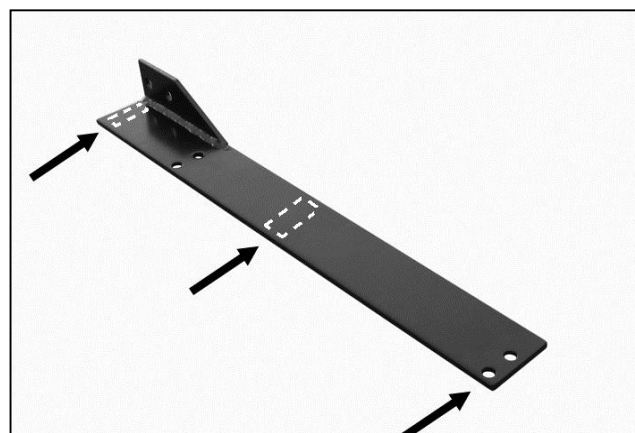
(Fig 7) If the forward hole in the Bracket does not line up with the stake pocket or the J Bolt will not fit properly, drill the necessary holes and bolt the Bracket directly to the top of the bed.
