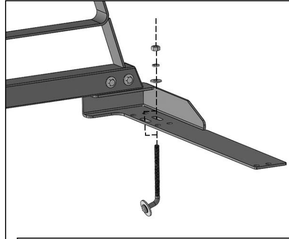
(Fig 4) Use the 10mm J-Bolt to secure the front mounting holes on the Bracket to the stake pocket if possible. Do not drill any mounting holes until after all mounting locations are checked for clearance
