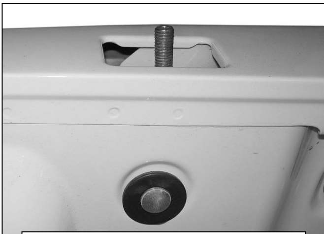
(Fig 5) Use the 10mm J-Bolt to secure the front mounting holes on the Bracket to the stake pocket if possible. Do not drill any mounting holes until after all mounting locations are checked for clearance
