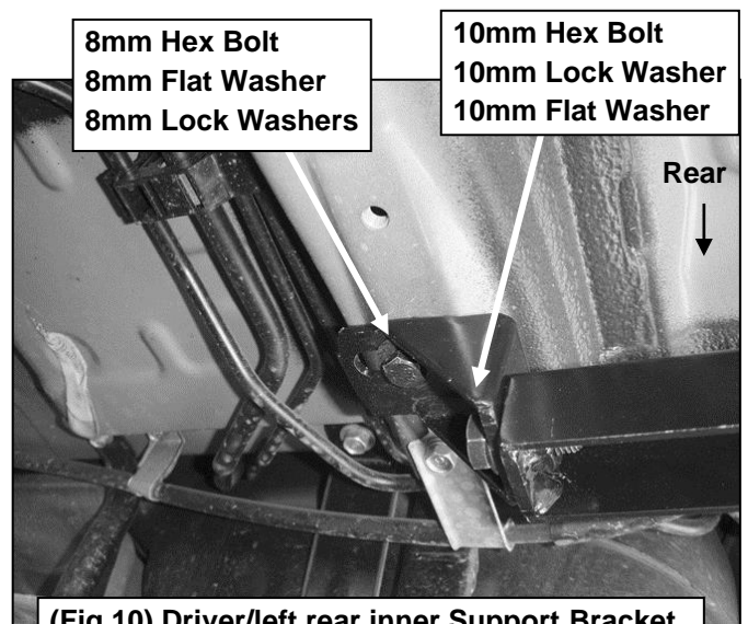
(Fig 10) Driver/left rear inner Support Bracket
